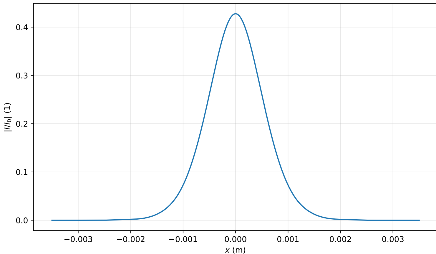
Intensity profile I(x, y = 0, z = 3.742m)/I_0 , P_{in}=0.5P_{cr} , artificial time
